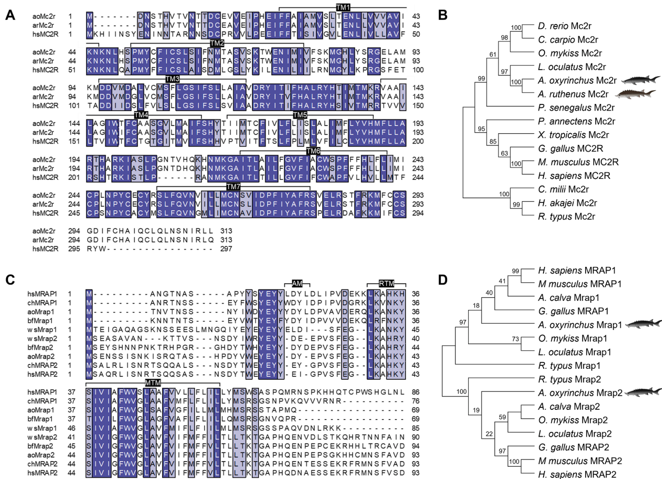
Fig. 1. Sequence alignment and phylogenetic comparisons of sturgeon Mc2r and Mrap1. (A) Alignment of Atlantic (ao) and sterlet (ar) sturgeon Mc2rs with human (hs) MC2R. The 7 transmembrane (TM) domains are labeled. (B) Molecular phylogeny of sturgeon Mc2rs among gnathostome Mc2rs. The clade of Chondrichthyes was rooted as an outgroup. (C) Alignment of Atlantic sturgeon (ao) Mrap1 with Mrap1s from a selection of jawed vertebrates: human (hs), chicken (ch), bowfin (bf), and whale shark (ws). The activation motif (AM), reverse topology motif (RTM), and the membrane trafficking motif (MTM) are labeled. (D) Molecular phylogeny of aoMrap1 among gnathostome Mraps. In Panels A and C, shading indicates identical (dark) and similar (light) residues. In Panels B and D, numbers indicate bootstrap values (1000 replicates). See Materials and Methods for details of analyses and sequence accession numbers.
