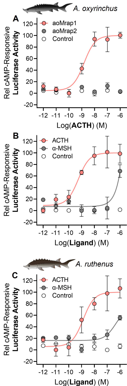
Fig. 3. Pharmacology of sturgeon Mc2r co-expressed with sturgeon Mrp1. (A) Dose-response stimulation by human (h) ACTH(1–24) of Atlantic sturgeon (ao) Mc2r co-expressed without an Mrp1 (Control) or with either aoMrp1 or Mrp2. (B–C) Dose-response stimulation by hACTH(1–24) or α-MSH of Atlantic sturgeon Mc2r (B) and sterlet sturgeon (C) co-expressed without (Control) or with aoMrp1. Data are presented as mean ± standard error ( n = 3 ) and lines represent fitted dose-response curve (three-parameter polynomial).
