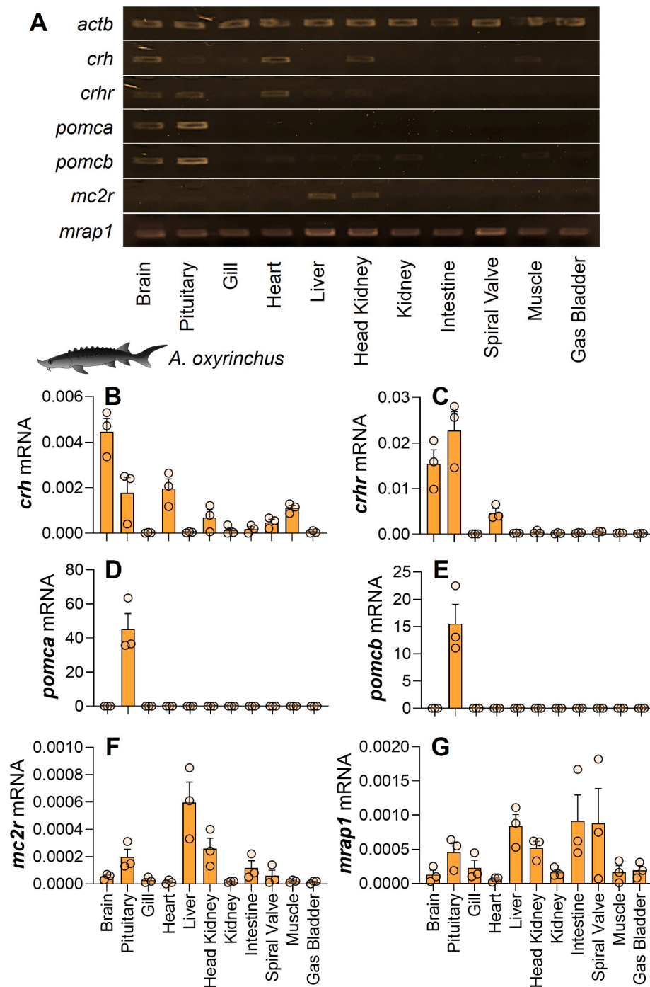
Fig. 4. Transcription profiles of HPI axis genes in Atlantic sturgeon. Tissue profiles of an a priori selection of genes classically understood to be involved in an HPI axis are presented as PCR products (A) and quantitative relative gene expression (B-G). Relative mRNA expression is presented as 2^{-\Delta CT} using several reference genes ( actb , gapdh , and ef1a ). Data are presented as mean \pm standard error. See text for gene names/abbreviations.
