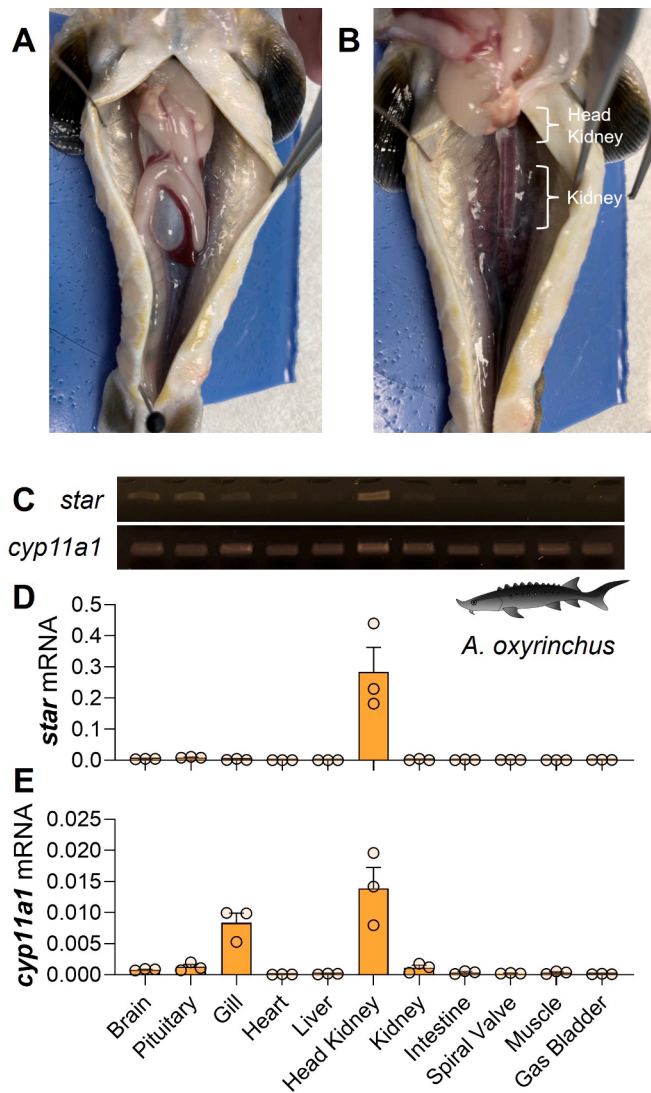
Fig. 5. Absence of yellow corpuscles and head kidney expression of star in Atlantic sturgeon. (A-B) Representative images of a dissection of Atlantic sturgeon body cavity with some internal organs in place (A) and removed (B) demonstrating the absence of yellow corpuscles along the dorsal body wall. For comparison, see white sturgeon dissection images presented by Kusakabe et al. (2009). (C-E) Tissue profile of star and cyp11a1 are presented as PCR products (C) and relative mRNA expression ( 2^{-\Delta CT} ) using several reference genes ( actb , gapdh , and e1a ) (D-E). Data are presented as mean \pm standard error. (For interpretation of the references to colour in this figure legend, the reader is referred to the web version of this article.)
