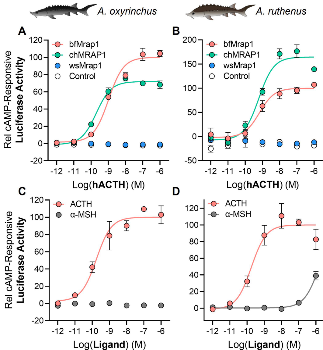
Fig. 2. Pharmacology of sturgeon Mc2r co-expressed with vertebrate Mrap1s. Pharmacology of Mc2r of two sturgeons are described: (A,C) Atlantic sturgeon and (B, D) sterlet sturgeon. (A-B) Dose-response stimulation by human (h) ACTH(1–24) of sturgeon Mc2rs co-expressed without (Control) or with various vertebrate Mrap1s: bowfin (bf), chicken (ch), whale shark (ws). (C-D) Dose-response stimulation by either ACTH or \alpha -MSH of sturgeon Mc2rs co-expressed with bfMrap1. Data are presented as mean \pm standard error ( n = 3 ) and lines represent fitted dose–response curve (three-parameter polynomial).
